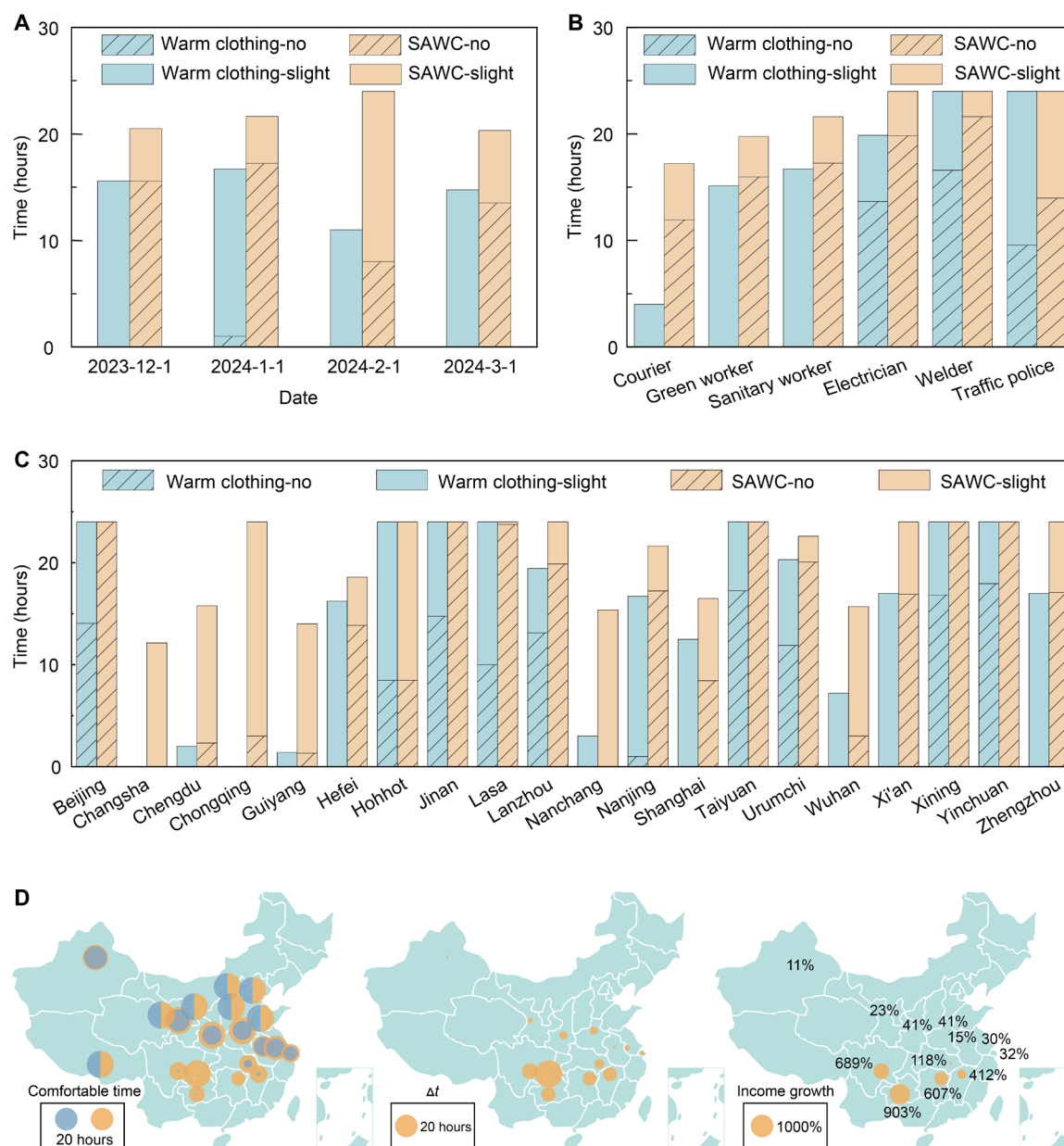
Fig. 5. Modeled comfortable time and income growth for urban outdoor workers. (A) The comparison of comfort time per day between sanitary workers with warm clothing and SAWC on different dates. The comfort time is the sum of the slight cold stress ( -1.5 to -0.5 ), no thermal stress ( -0.5 to 0.5 ), and slight heat stress zone ( 0.5 to 1.5 ). The blue (Warm clothing-no) and orange colors (SAWC-no) with patterns represent the no thermal stress zone of workers with warm clothing and SAWC, respectively. The blue (Warm clothing-slight) and orange colors (SAWC-slight) without patterns represent the sum of slight cold and heat stress zones of workers with warm clothing and SAWC, respectively. (B) The comparison of comfort time of different workers in Nanjing on 1 January 2024. (C) The comparison of comfort time for sanitary workers in different cities on 1 January 2024. (D) The comfort time (left), its difference (mid), and income growth (right) of sanitary workers with warm clothing and SAWCs in 20 cities in China on 1 January 2024. The blue and orange circles in the left map represent the comfort time of sanitary workers with warm clothing and SAWCs, respectively. The circles composed of a blue semicircle and an orange semicircle represent the comfort time that is 24 hours for sanitary workers with warm clothing and SAWCs. The values are scaled to the diameter of the circle.
